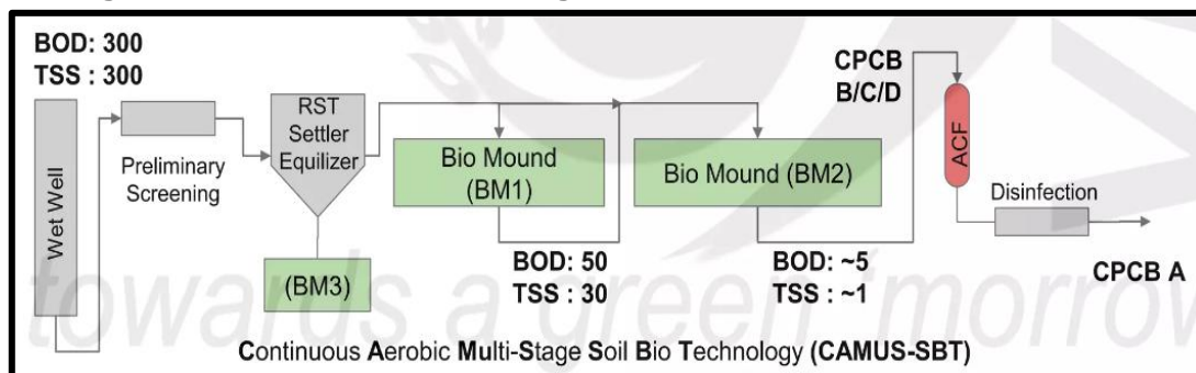
Figure 3: STP Process Flow Diagram and SBT – Water Balance for Site
