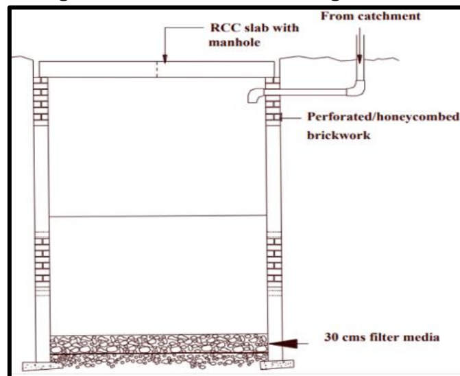
Figure 4 : Rainwater Harvesting Structure
